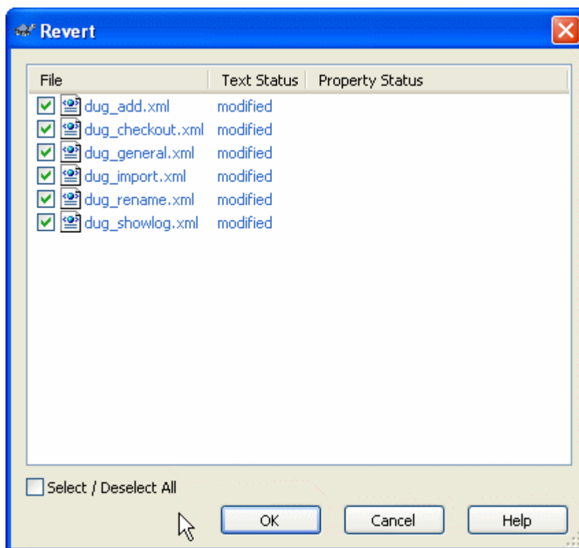
Figure 4.30. Revert dialog
